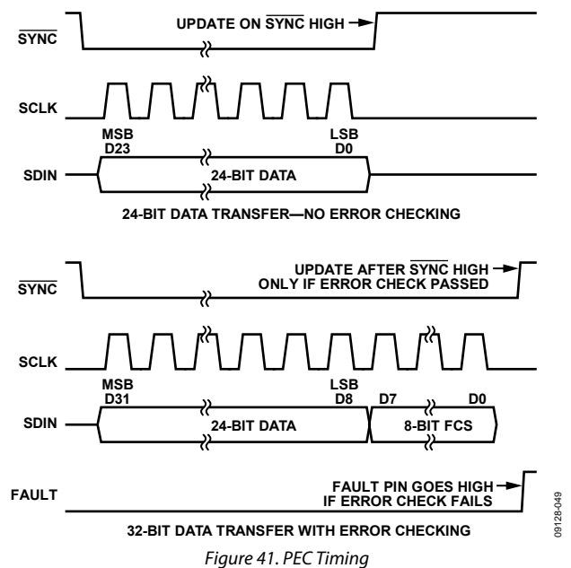
Figure 41. PEC Timing
