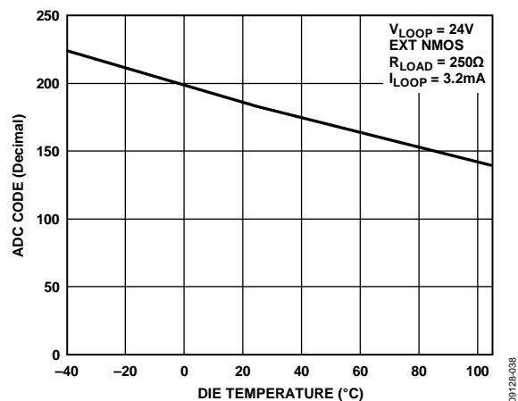
Figure 39. On-Chip ADC Code vs. Die Temperature
