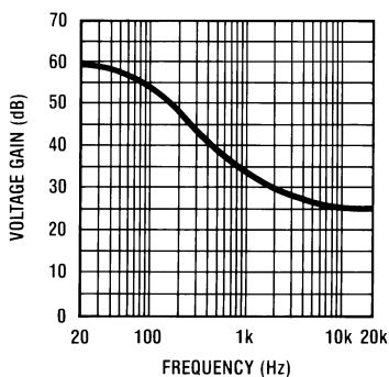
Figure 84. NAB Preamplifier Voltage Gain vs Frequency V_{IN} = 10\text{mV} , 34.5\text{dB} , f = 1\text{kHz}
