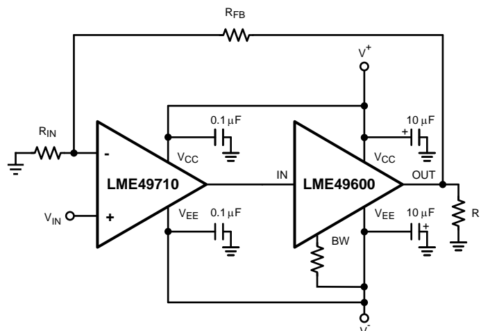
Figure 26. High Performance, High Fidelity LME49600 Audio Buffer Application
